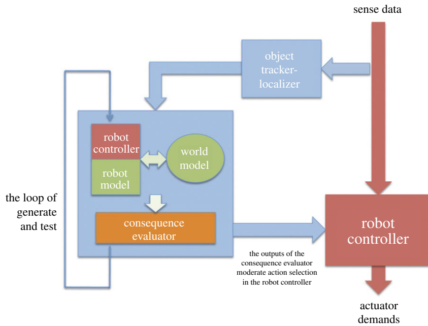
Figure 4. Block diagram of a robot equipped with a consequence engine. The robot control dataflows are shown in red (right); the consequence engine and its dataflows in blue (left). Adapted from Winfield [27].
